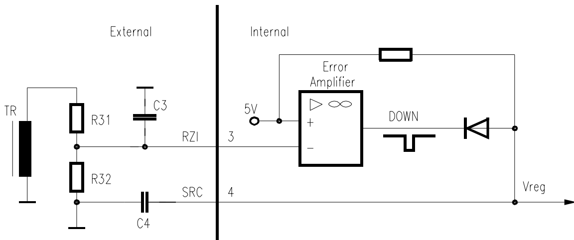
Figure 9 Error Amplifier
