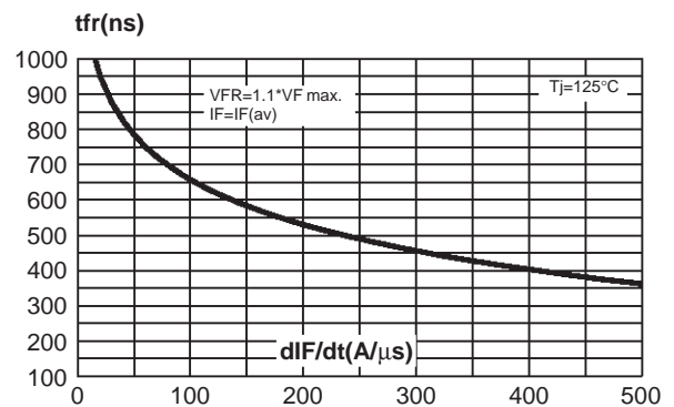
Fig. 201: Forward recovery time versus dI_F/dt (90% confidence, per diode).
