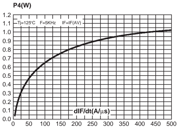
Fig. 11: Switching ON losses versus dI/dt .
