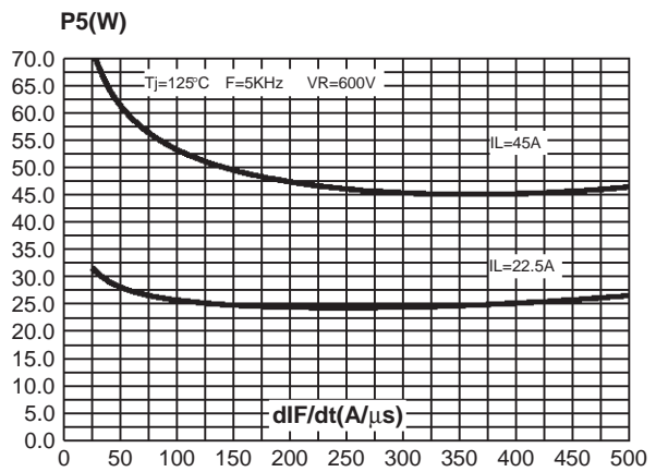
Fig. 12: Switching losses in transistor due to the diode.
