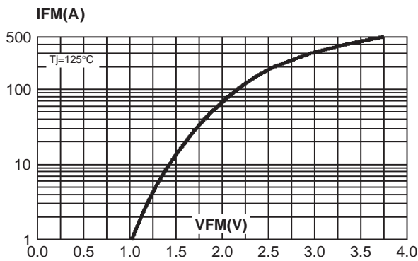
Fig. 13: Forward voltage drop versus forward current (maximum values, per diode).
