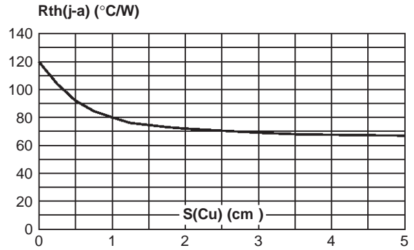
Fig. 8-2: Thermal resistance junction to ambient versus copper surface under each lead (Epoxy printed circuit board FR4, copper thickness: 35µm) (SMA).
