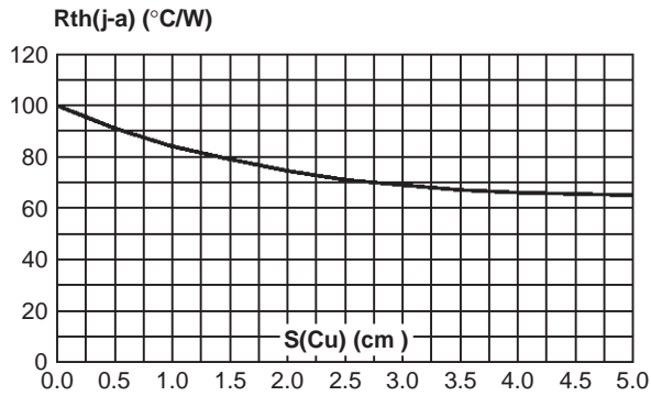
Fig. 8-1: Thermal resistance junction to ambient versus copper surface under tab (Epoxy printed circuit board FR4, copper thickness: 35µm) (SMB).
