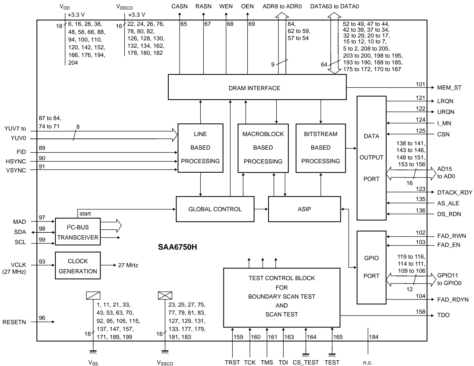
Fig.1 Block diagram.
