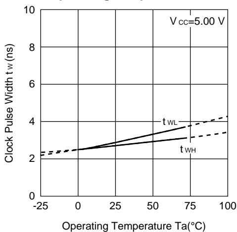
Figure 23 Clock Pulse Width vs. Operating Temperature
