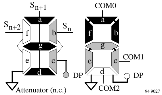
Figure 39. 3:1 multiplex 7 segment digit
