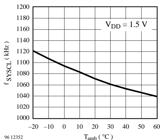
Figure 49. SYSCl = f(T_{amb}) - 1.5V option
