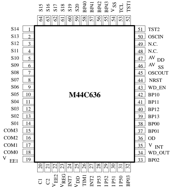
Figure 54. M44C636 in 64 pin plastic QFP (top view)
