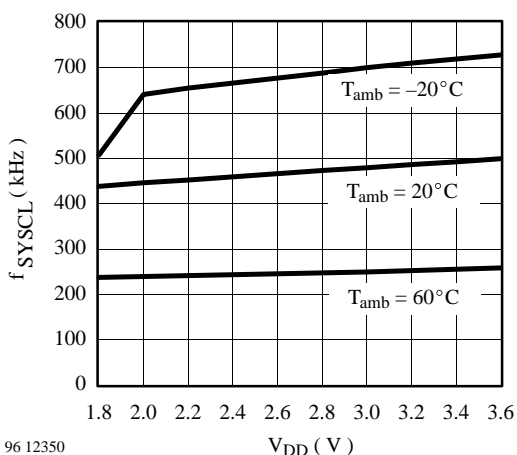
Figure 47. SYSCl = f(V_{DD}, T_{amb}) - 3V option
