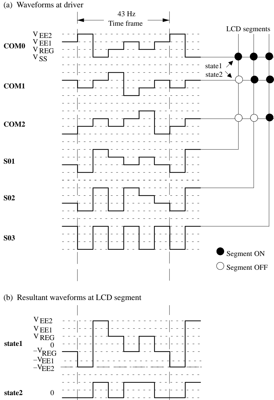
Figure 41. Waveforms for 3:1 multiplex drive mode
