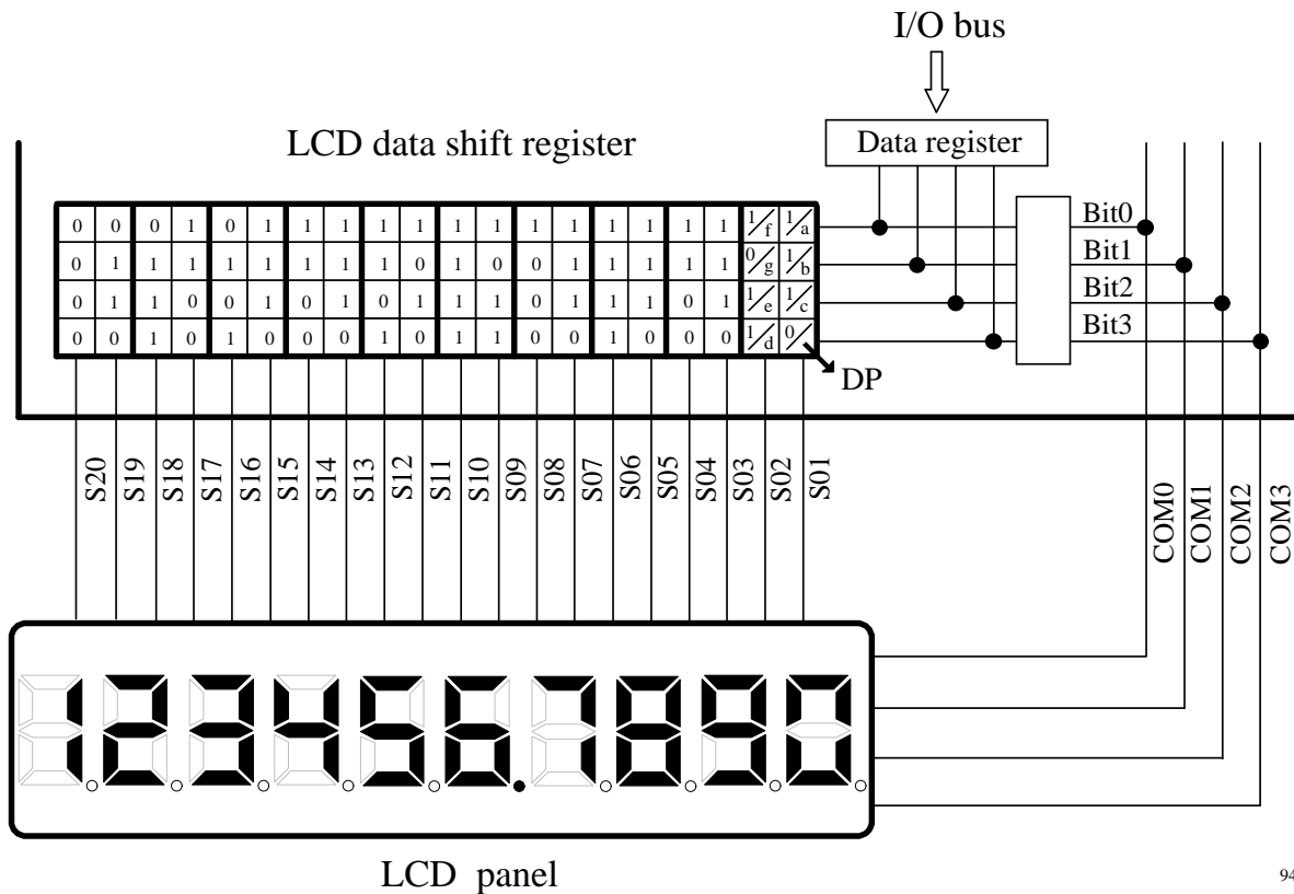
Figure 43. 4:1 multiplex LCD panel connection
