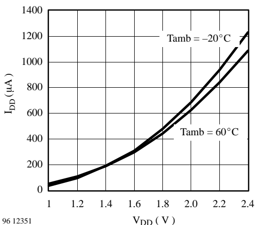
Figure 48. I_{DD} = f(V_{DD}, T_{amb}) - 1.5V option
