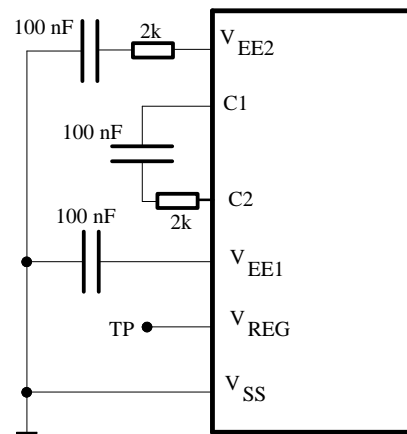
Figure 34. External components
