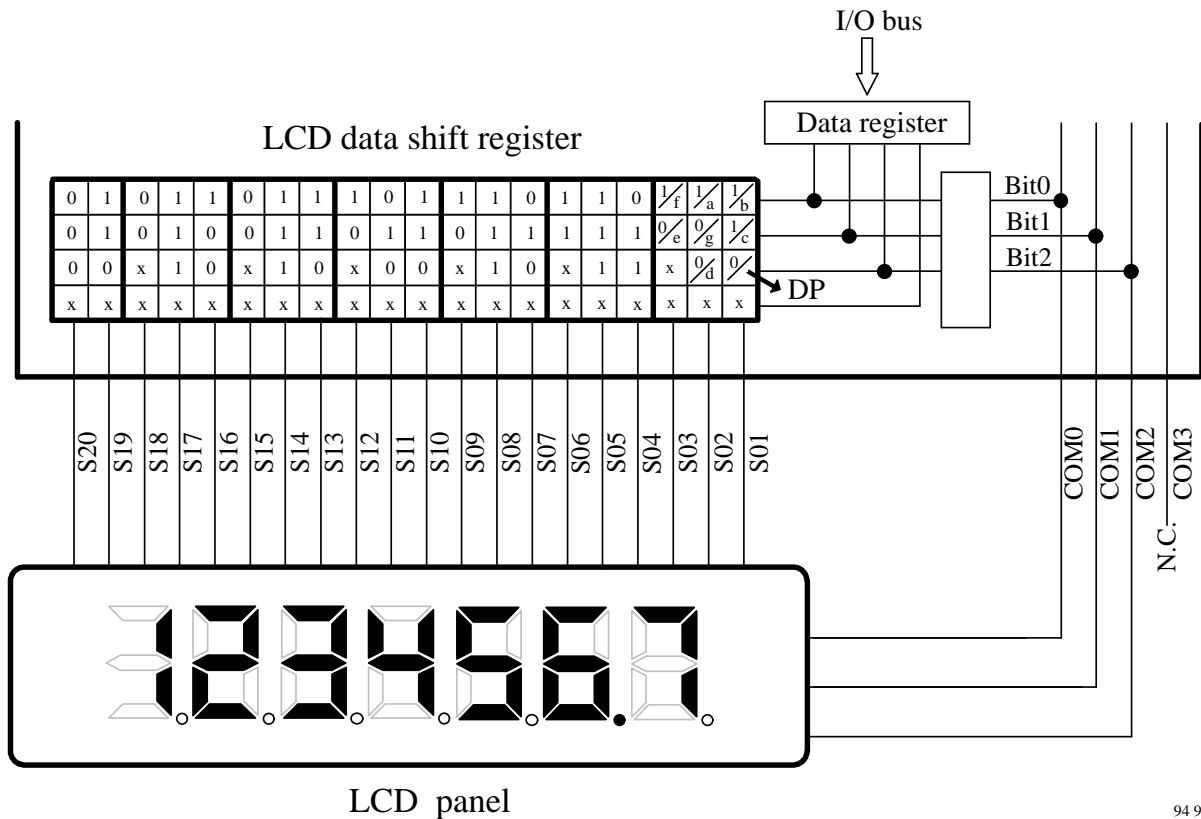
Figure 40. 3:1 multiplex LCD panel connection
