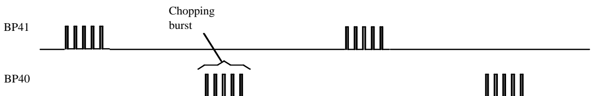
Figure 23. Motor driver output waveforms
