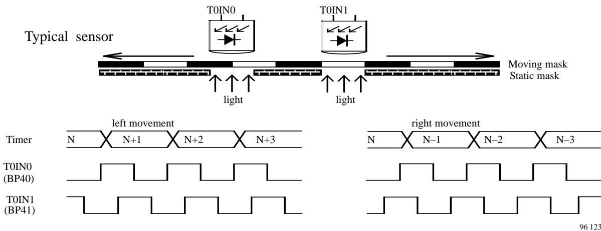
Figure 29. Position measurement mode
