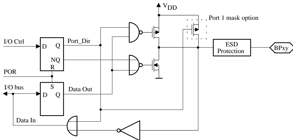
Figure 5. Bidirectional Port 0 and 1 schematics
