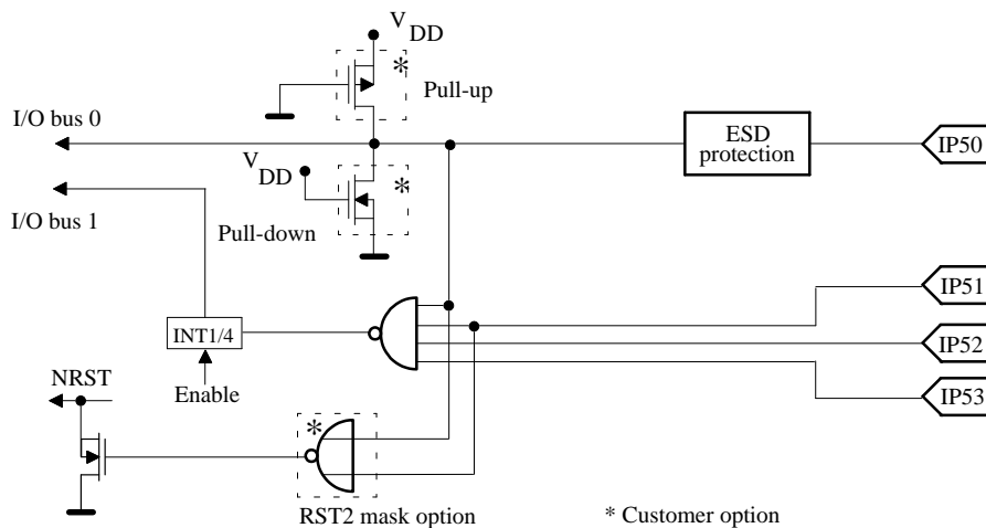
Figure 8. Port 5 with pull-up and RST2 mask option
