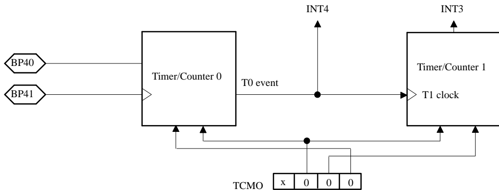
Figure 32. Timer/counter 16-bit mode (running condition)
