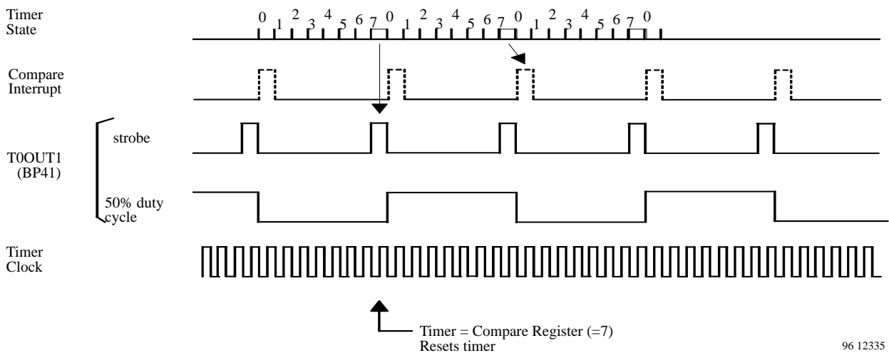
Figure 21. Timer 0 counter reload mode
