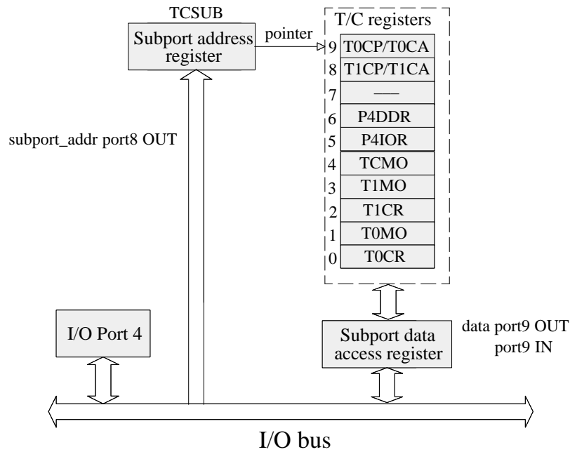
Figure 18. Timer/Counter extended I/O addressing
