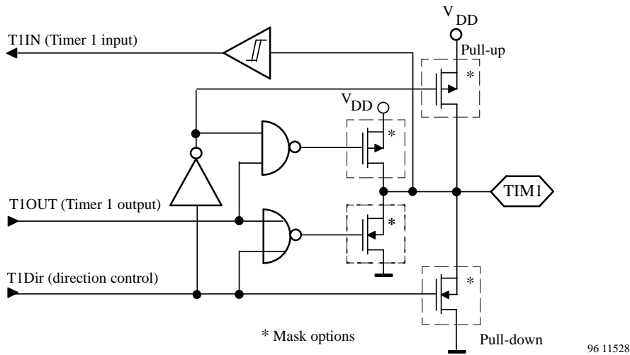
Figure 4. Bidirectional pin TIM1
