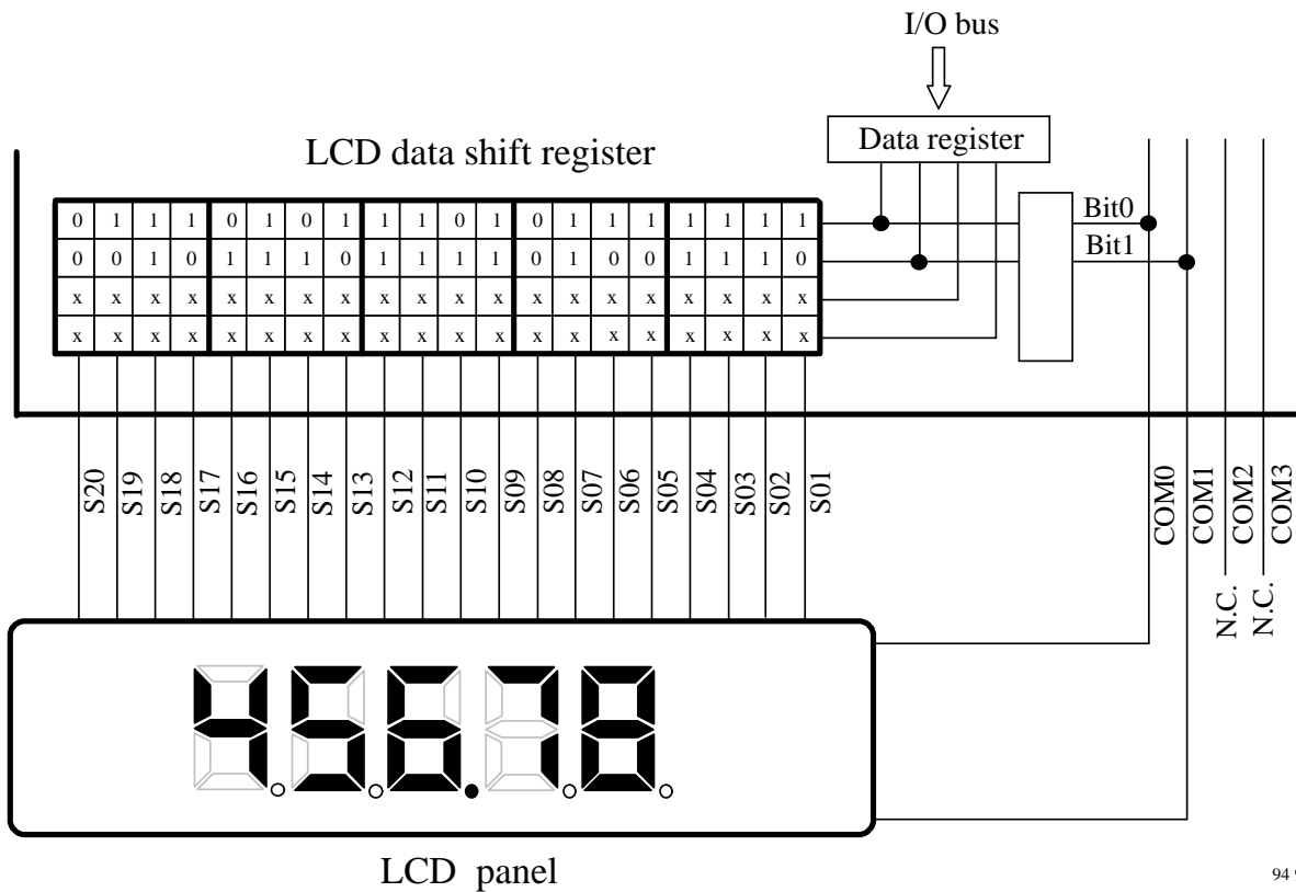
Figure 37. 2:1 multiplex LCD panel connection
