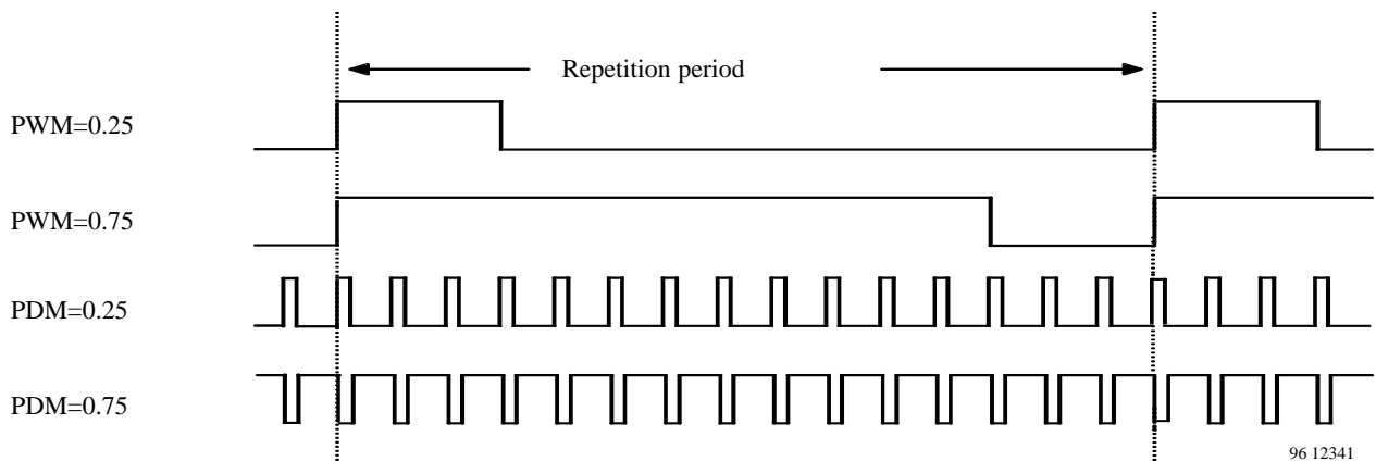
Figure 27. An example 4-bit PWM/PDM comparison
