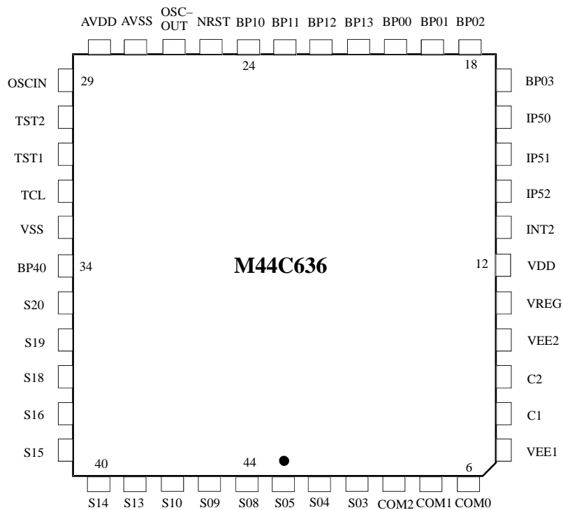
Figure 55. M44C636 in 44 pin PLCC (top view)
