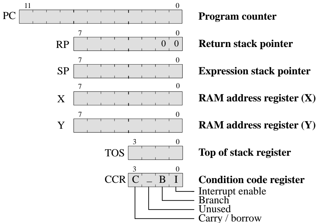
Figure 10. Programming model
