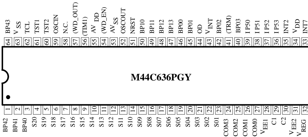
Figure 53. Pin-out of M44C636 piggyback and target board adapter
