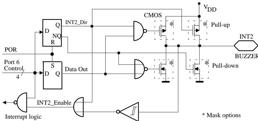
Figure 16. External interrupt INT2 and BUZZER output
