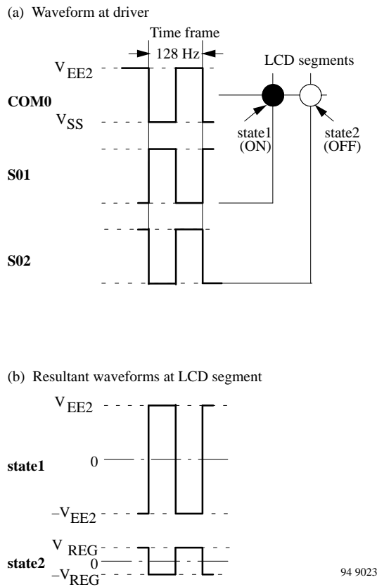
Figure 35. Direct drive mode waveforms
