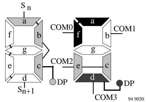
Figure 42. 4:1 multiplex 7 segment digit
