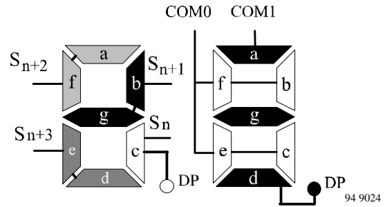
Figure 36. 2:1 multiplex 7 segment digit
