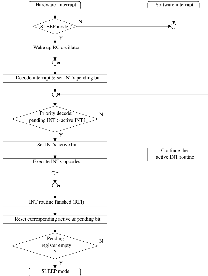
Figure 13. Interrupt flowchart
