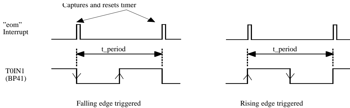
Figure 30. Period measurement
