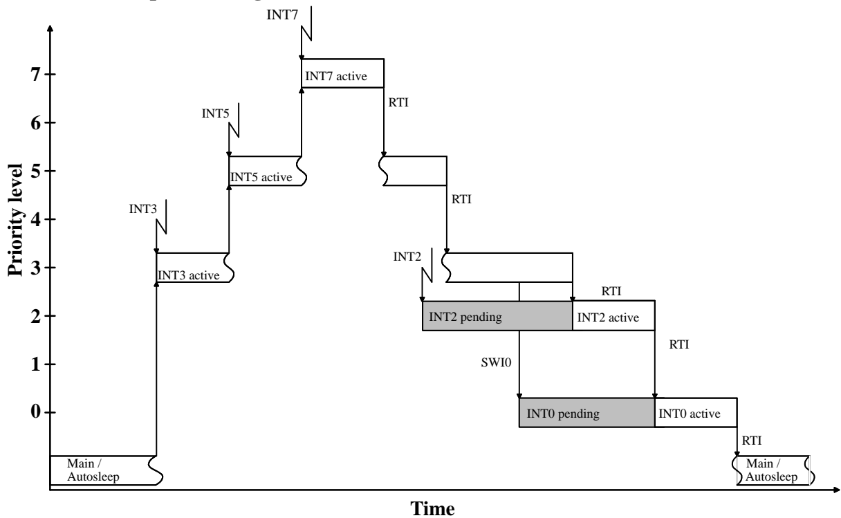
Figure 14. Interrupt processing
