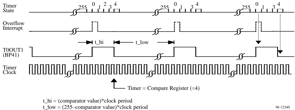
Figure 26. Timer 0 pulse width modulation
