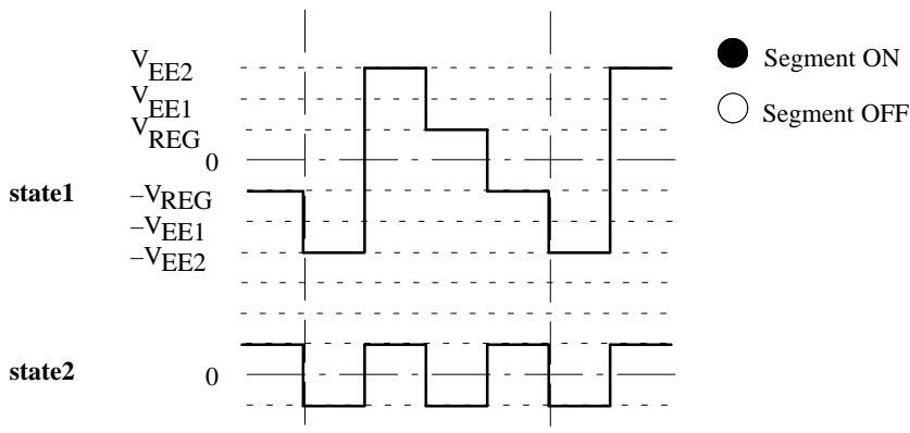
Figure 38. Waveforms for 2:1 multiplex drive mode
