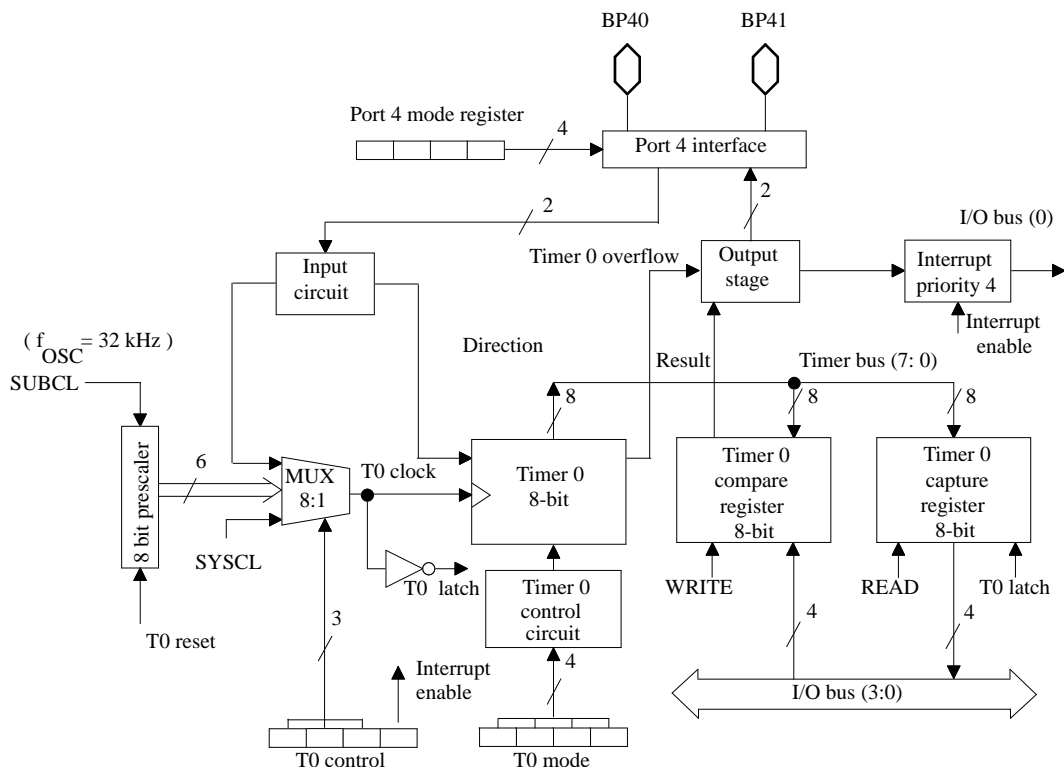
Figure 19. Timer 0 block diagram
