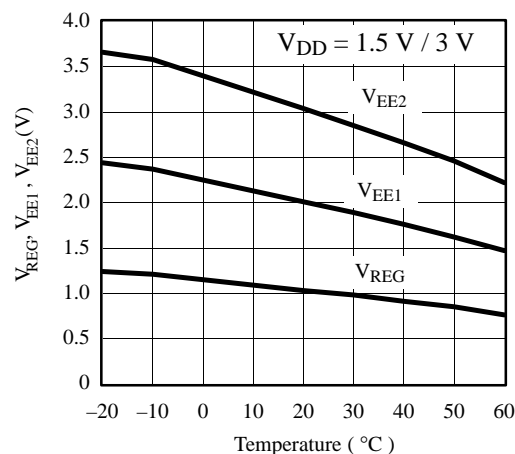
Figure 51. LCD voltages vs. temperature
