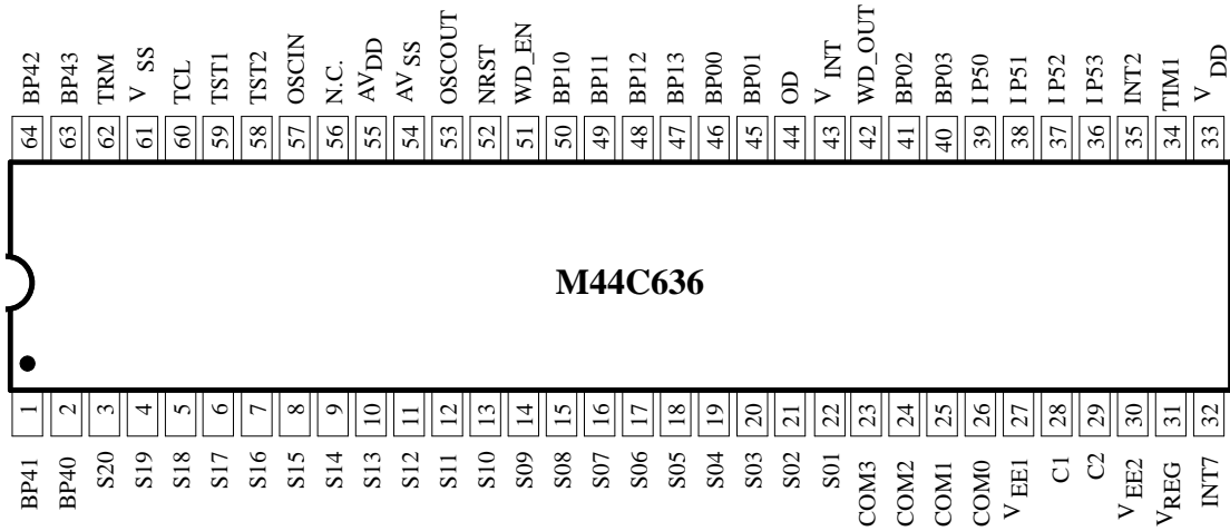
Figure 52. Emulation package – 64 pin ceramic DIL
