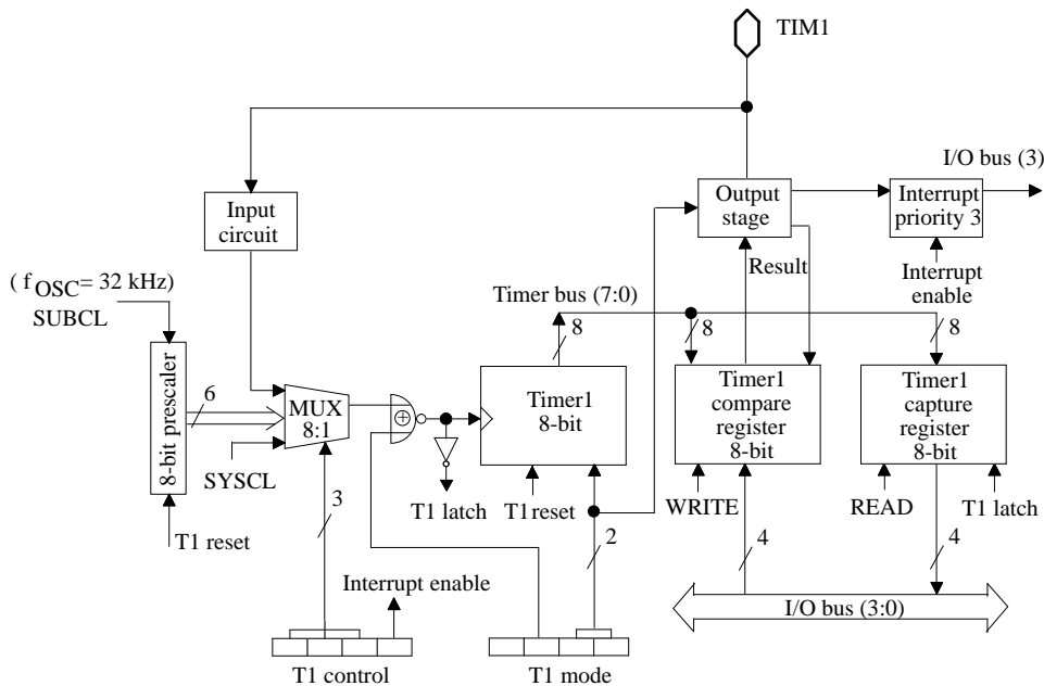
Figure 31. Block diagram of Timer 1
