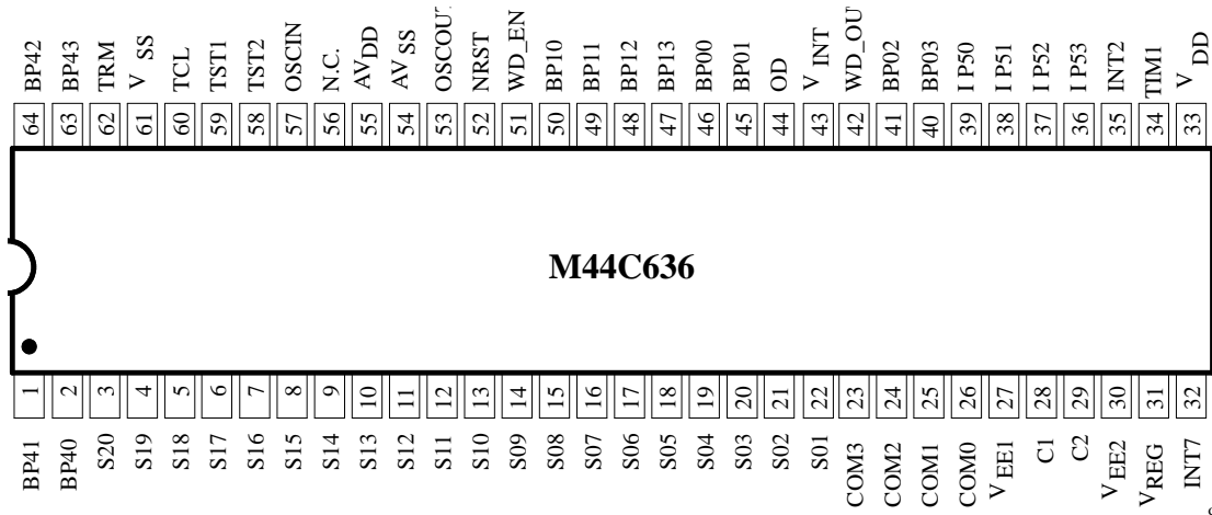
Figure 2. Pin connection – 64 pin ceramic DIL
