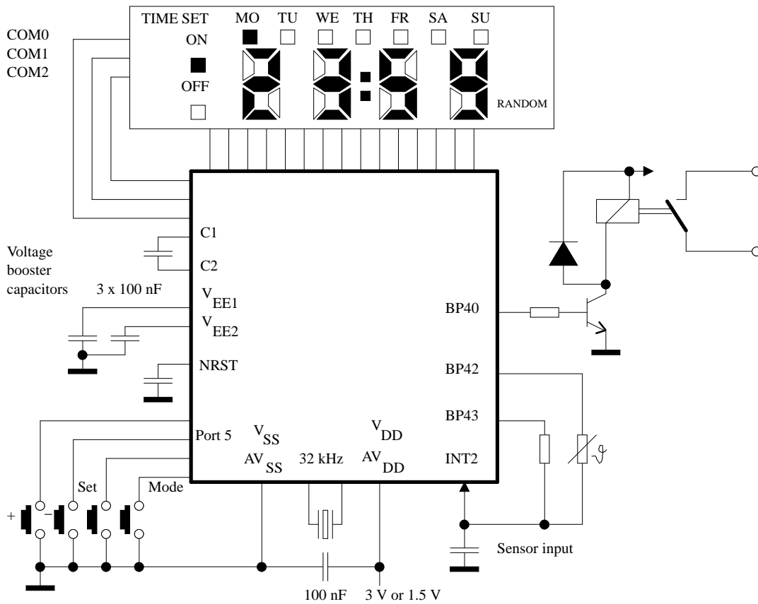
Figure 57. Application example
