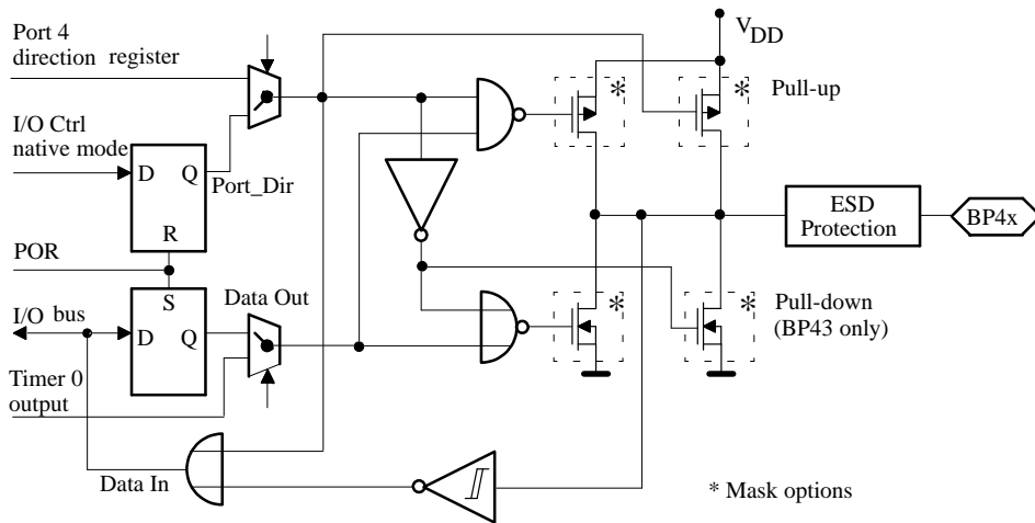
Figure 7. Bidirectional Port 4 schematics
