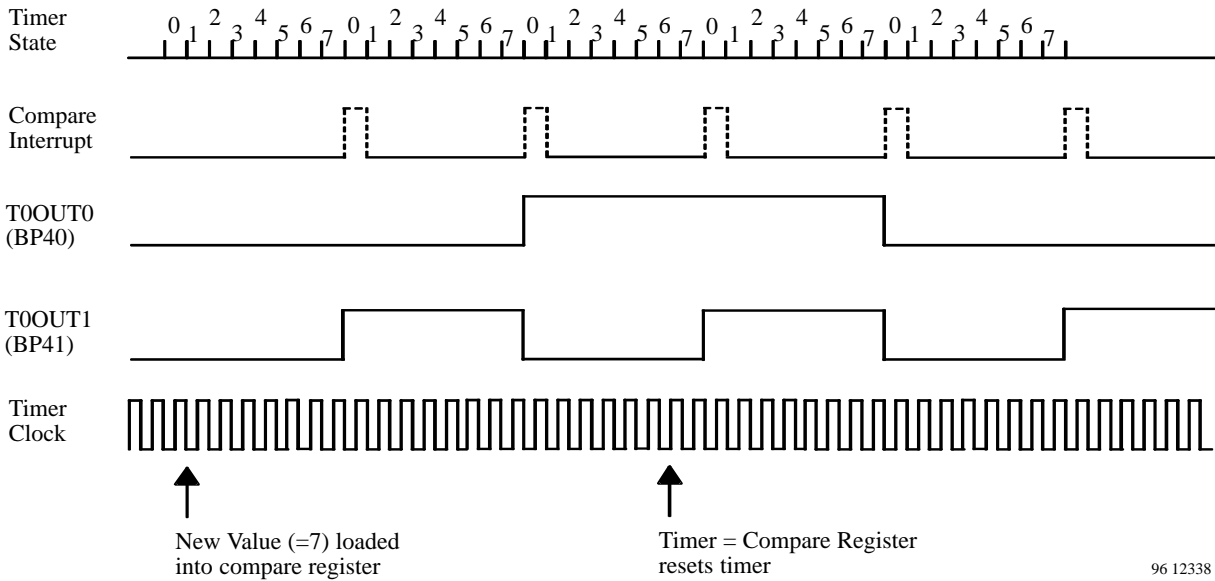
Figure 24. Modulated melody mode
