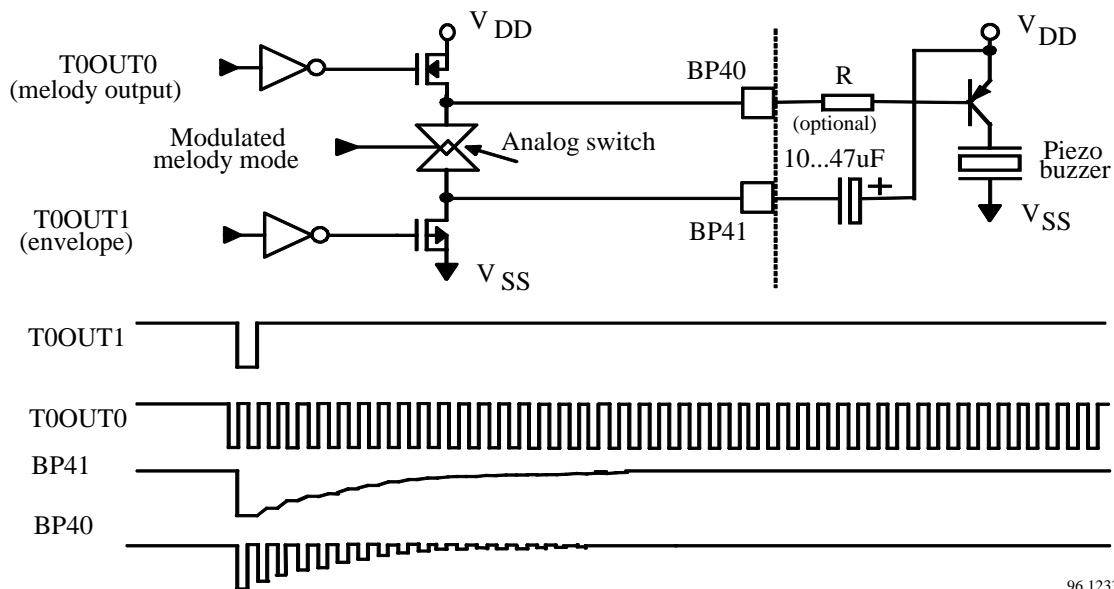
Figure 25. Modulated melody output circuit
