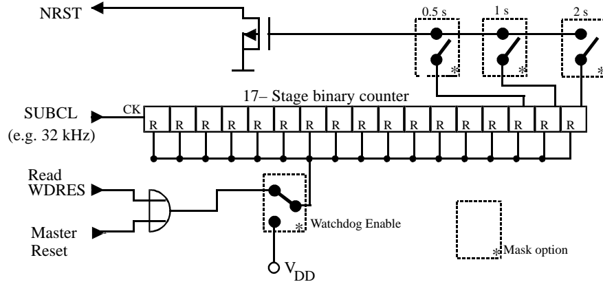
Figure 12. Watchdog timer
