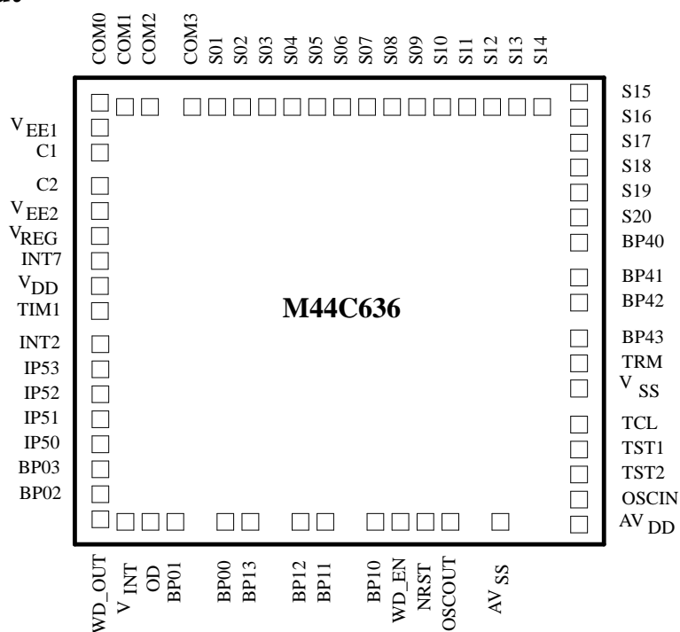
Figure 56. M44C636 pad configuration
