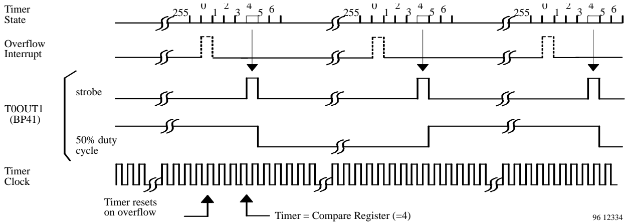
Figure 20. Timer 0 free running counter mode
