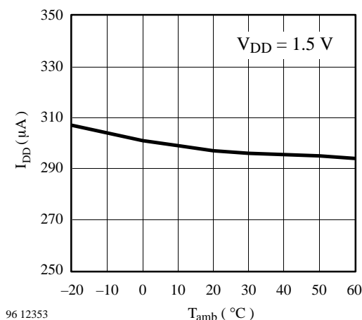
Figure 50. I_{DD} = f(T_{amb}) - 1.5V option
