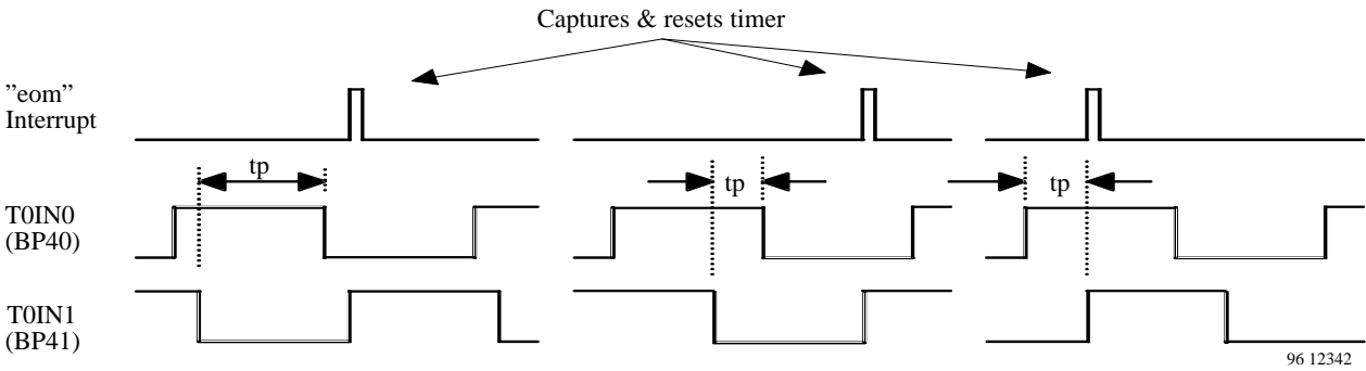
Figure 28. Phase measurement
