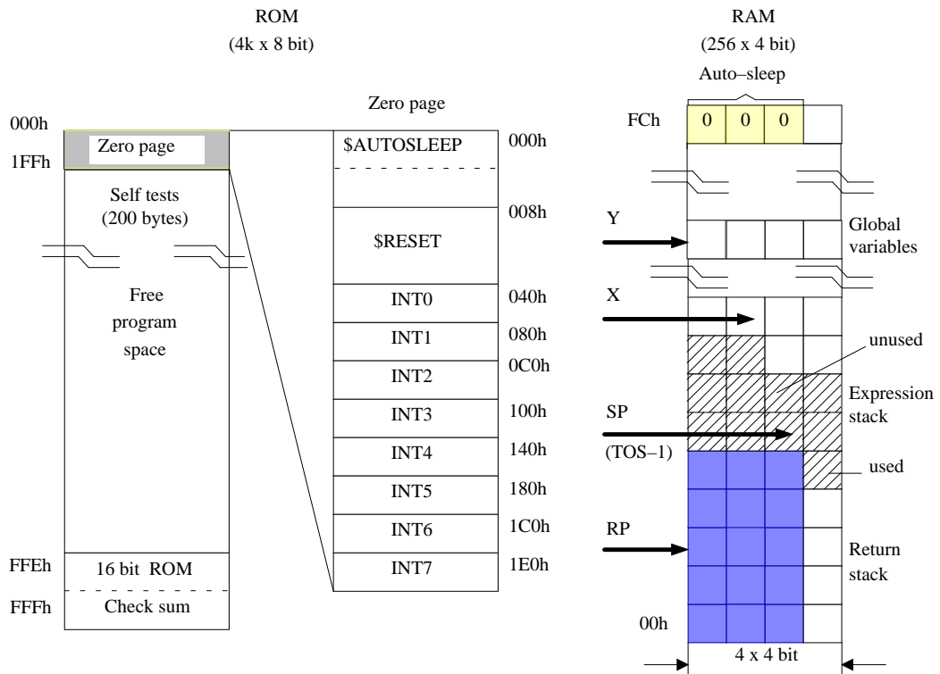
Figure 9. Memory map
