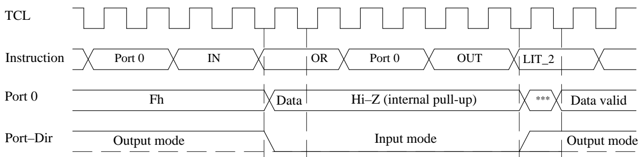
Figure 6. Port read and write cycle timing
