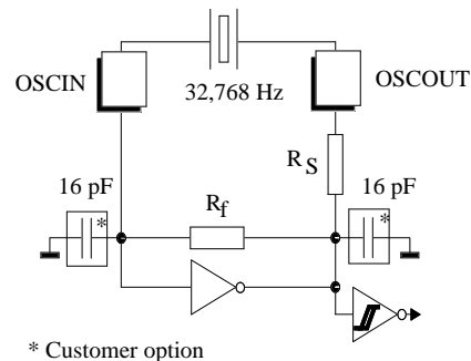
Figure 3. Crystal oscillator
