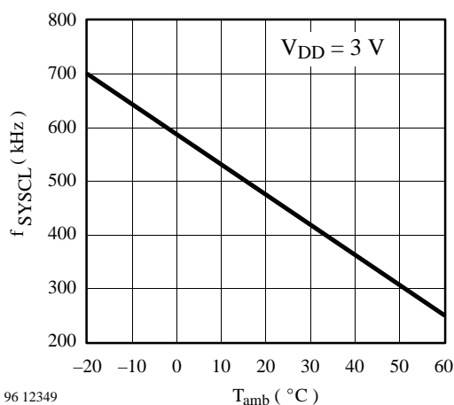
Figure 46. SYSCl = f(T_{amb}) - 3V option
