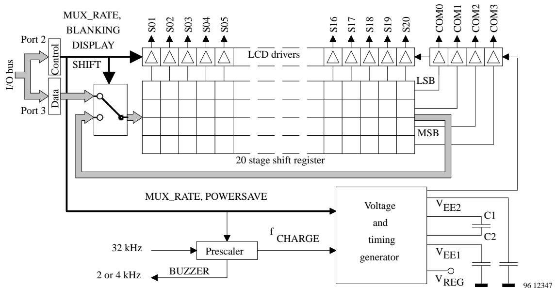
Figure 33. LCD driver – functional block diagram
