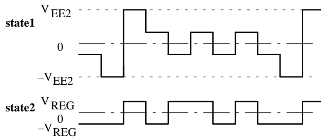
Figure 44. Waveforms for 4:1 multiplex drive mode
