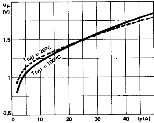
Figure 5. Voltage drop versus forward current
