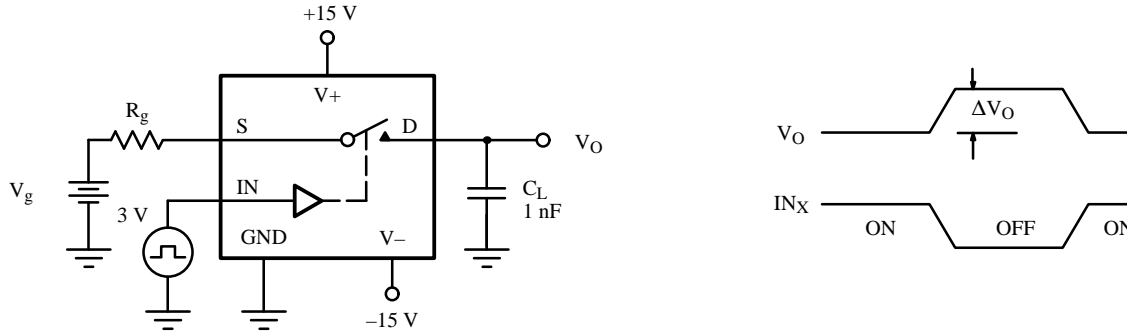
Figure 4. Charge Injection
