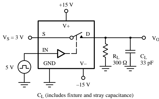
Figure 2. Switching Time
