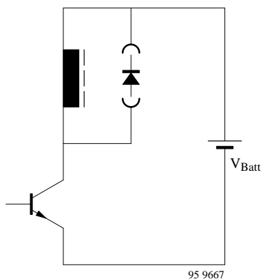
Figure 2. Test circuit
