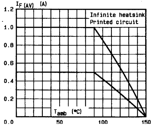
Figure 2. Average forward current versus average ambient temperature.
