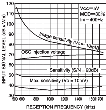
Fig. 14 Tracking characteristics
