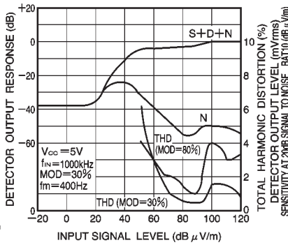
Fig. 21 Sensitivity characteristics
