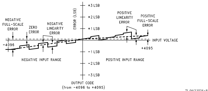
FIGURE 1c. Simplified Error Curve vs Output Code after Auto-Cal Cycle
