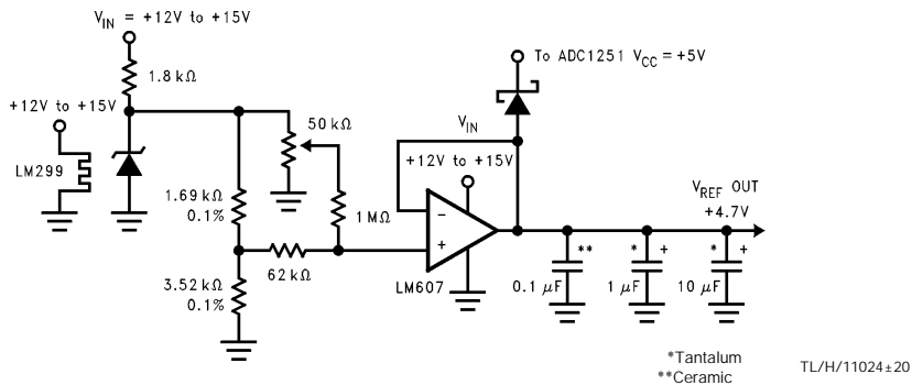
FIGURE 4. Low Drift Extremely Stable Reference Circuit
