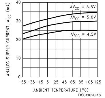
Analog Supply Current vs Temperature
