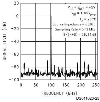
Spectral Response with 100 kHz Sine Wave Input
