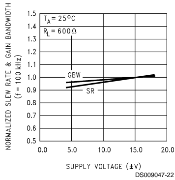
Normalized Slew Rate & Gain Bandwidth vs Supply Voltage (f = 100 kHz)
