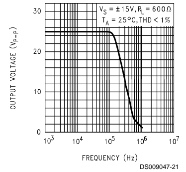
Power Bandwidth
