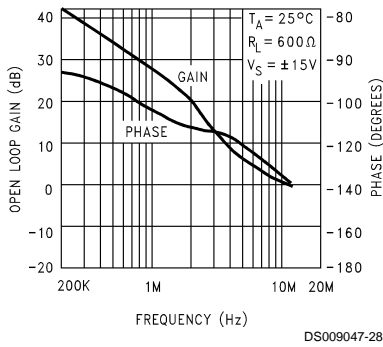
Open Loop Gain & Phase vs Frequency
