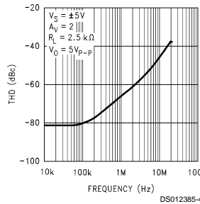
Total Harmonic Distortion vs Frequency (Note 13)
