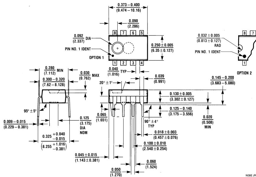
Order Number LM7171AIN or LM7171BIN 8-Lead (0.300" Wide) Molded Dual-In-Line Package, JEDEC NS Package Number N08E
