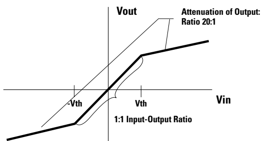
Figure 6: Input-output voltage profile of dual-slope attenuator
