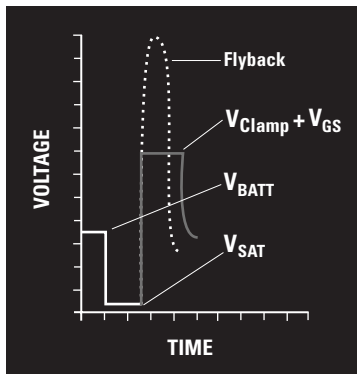
Figure 4: Voltage profile of solenoid deactivation
