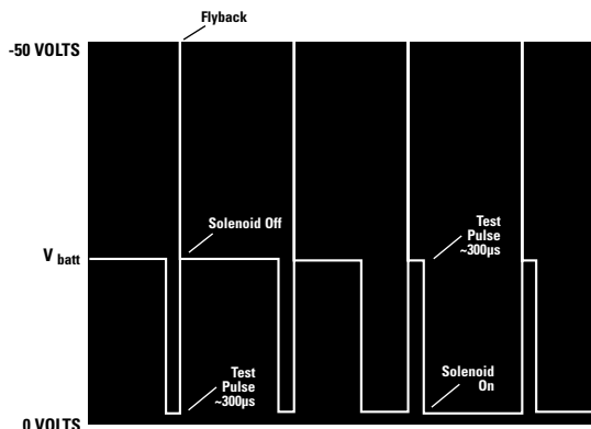
Figure 7: Test pulses applied regularly as a diagnostic input for determining ABS system integrity
