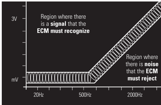
Figure 2: ABS/TC ECM response to VRS input
