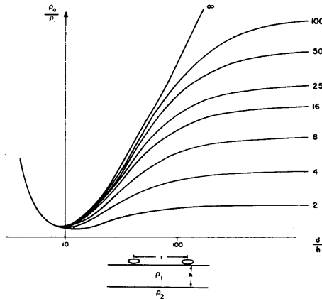
FIGURE 19(a). Two layer curves.
