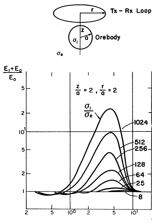
FIGURE 28. Combined response from orebody and conductive host rock (8).
