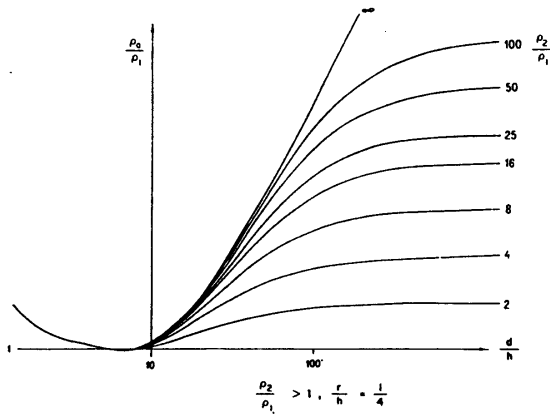
FIGURE 20. Two layer curves.
