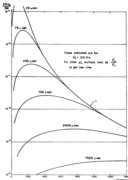
FIGURE 13. Current density - surface homogeneous half-space.
