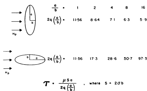
FIGURE 11. Time constant - infinite elliptical cylinder.
