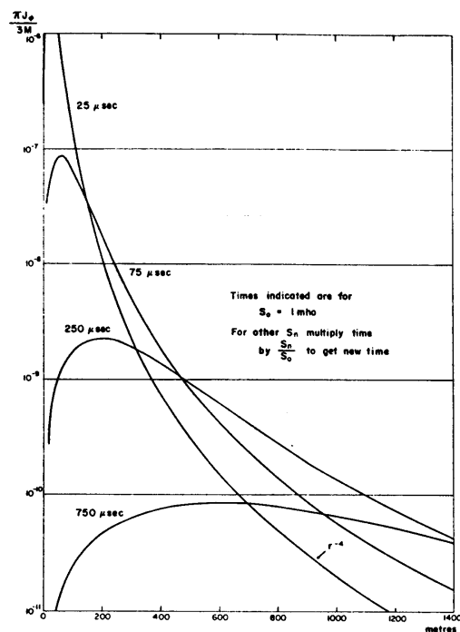
FIGURE 21. Current density – horizontal thin sheet.
