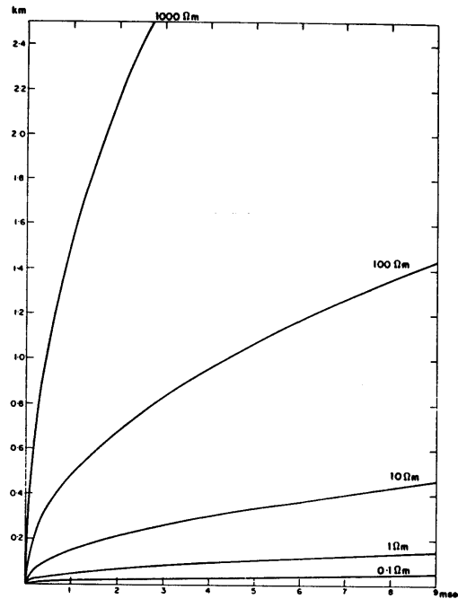
FIGURE 15. Location of surface current maximum—homogeneous half-space.
