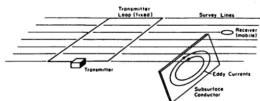
FIGURE 1. Survey configuration.
