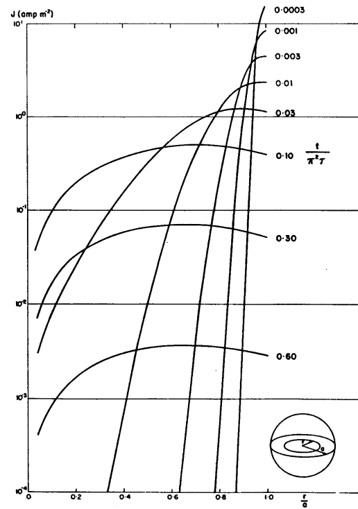
FIGURE 7. Radial distribution of sphere currents.
