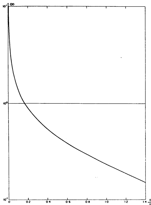
FIGURE 8. Time derivative of sphere secondary magnetic field.
