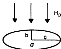
FIGURE 9. Oblate spheroid.
