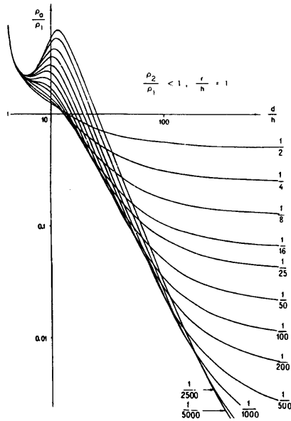
FIGURE 19(b). Two layer curves
