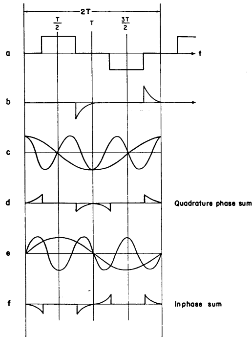
FIGURE 26. Synthesis of transient response.
