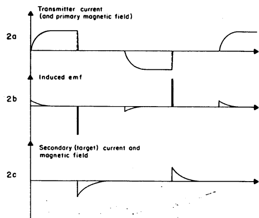
FIGURE 2. System waveforms.
